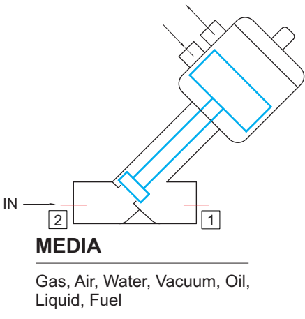
Normally close Pressure Below Seat
