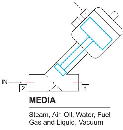
Normally open Pressure Below Seat
