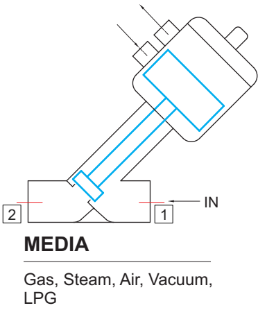
Normally close Pressure Above Seat
